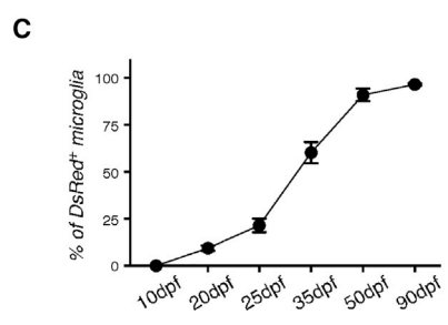
Figure 4. Kinetics of Adult MG Emergence during Zebrafish Development (A) Scheme of the transgenic lines used to discriminate pMF-derived embryonic MG from endothelial-derived adult MG. (B) GFP (left panels) and DsRed (middle panels) immunostaining performed on brain sections from Tg(kdr1:Cre; \beta actin:Switch-DsRed; mpeg1:GFP) triple transgenics at the indicated developmental stage, showing the replacement of GFP + DsRed - embryonic MG by GFP + DsRed + cells in the brain parenchyma. The right panels show a merge of both fluorescent channels. Scale bar: 50 \mu m.
